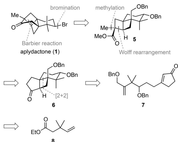
Scheme 1. Retrosynthetic analysis of aplydactone ( 1 ).
